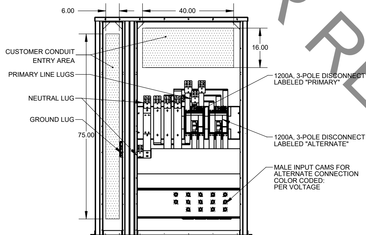
FRONT VIEW (DOOR AND DEADFRONT REMOVED)
