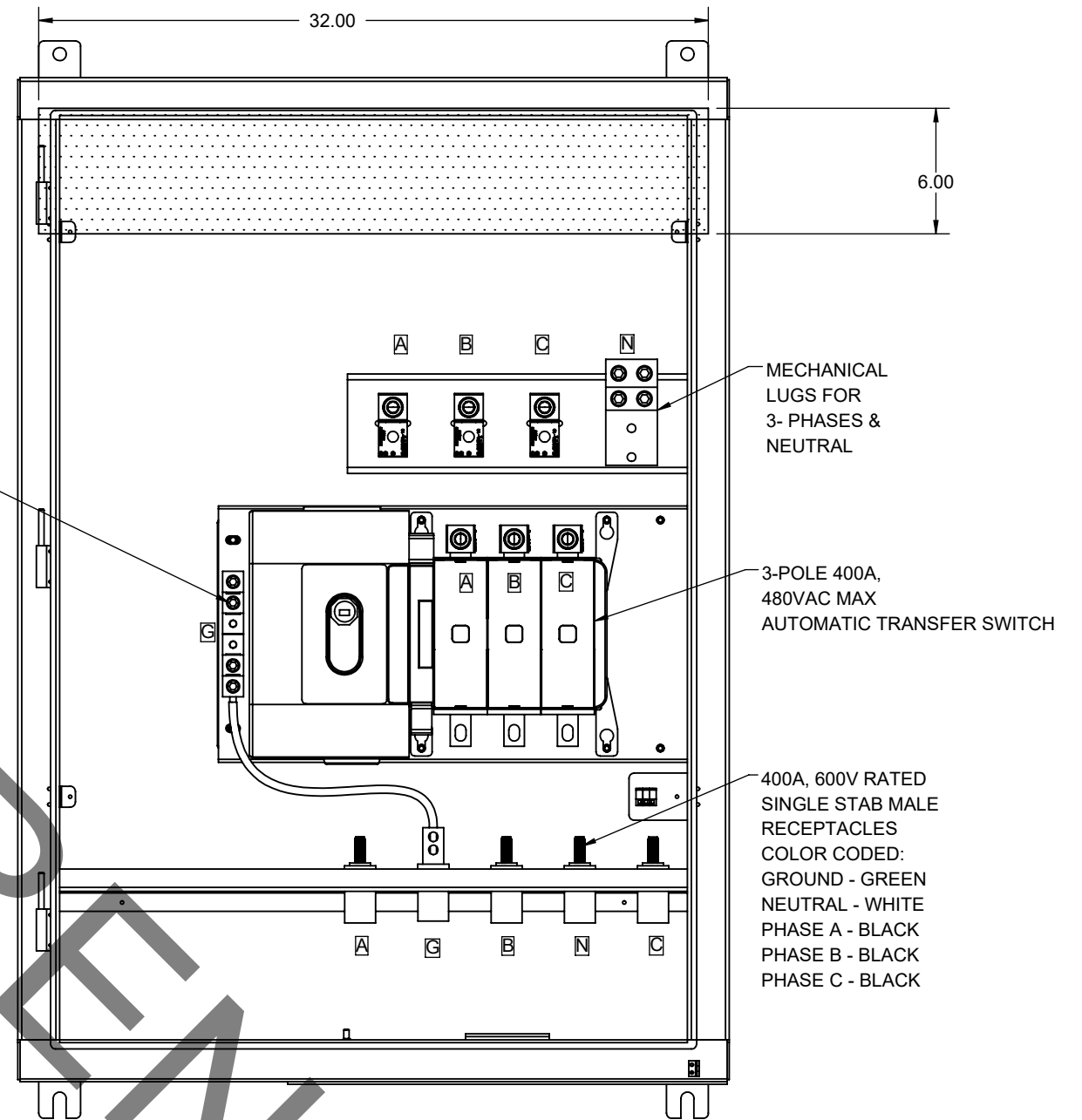
FRONT VIEW (DOOR & DEADFRONT NOT SHOWN)
