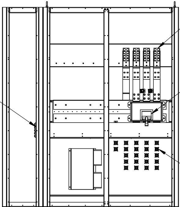
FRONT VIEW (DOORS AND DEADFRONTS REMOVED)
