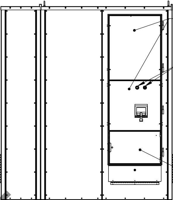
FRONT VIEW (DOORS REMOVED)
