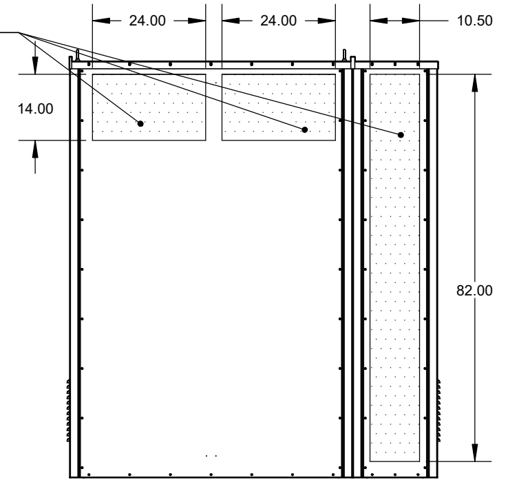
BACK VIEW
