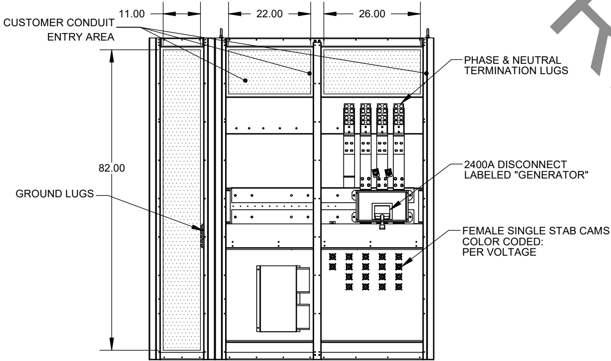
FRONT VIEW (DOORS AND DEADFRONTS REMOVED)
