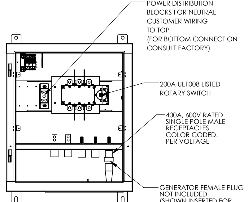
FRONT VIEW (DOOR AND DEADFRONT REMOVED)
