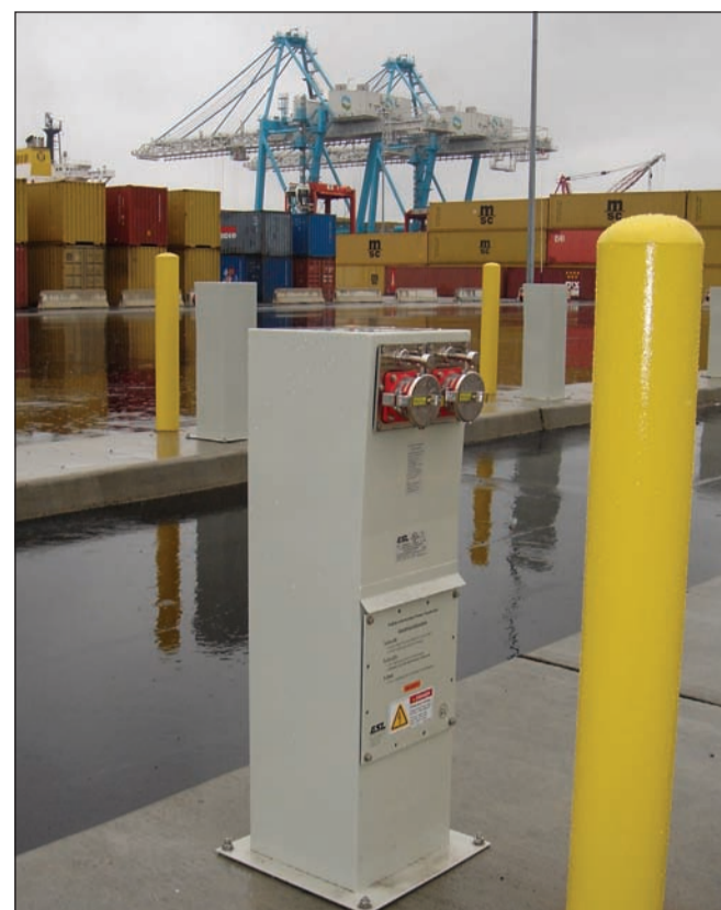
More and more terminal operators are opting for two and three-gang ROAs like this twin outlet assembly in a pedestal design for a straddle carrier terminal
