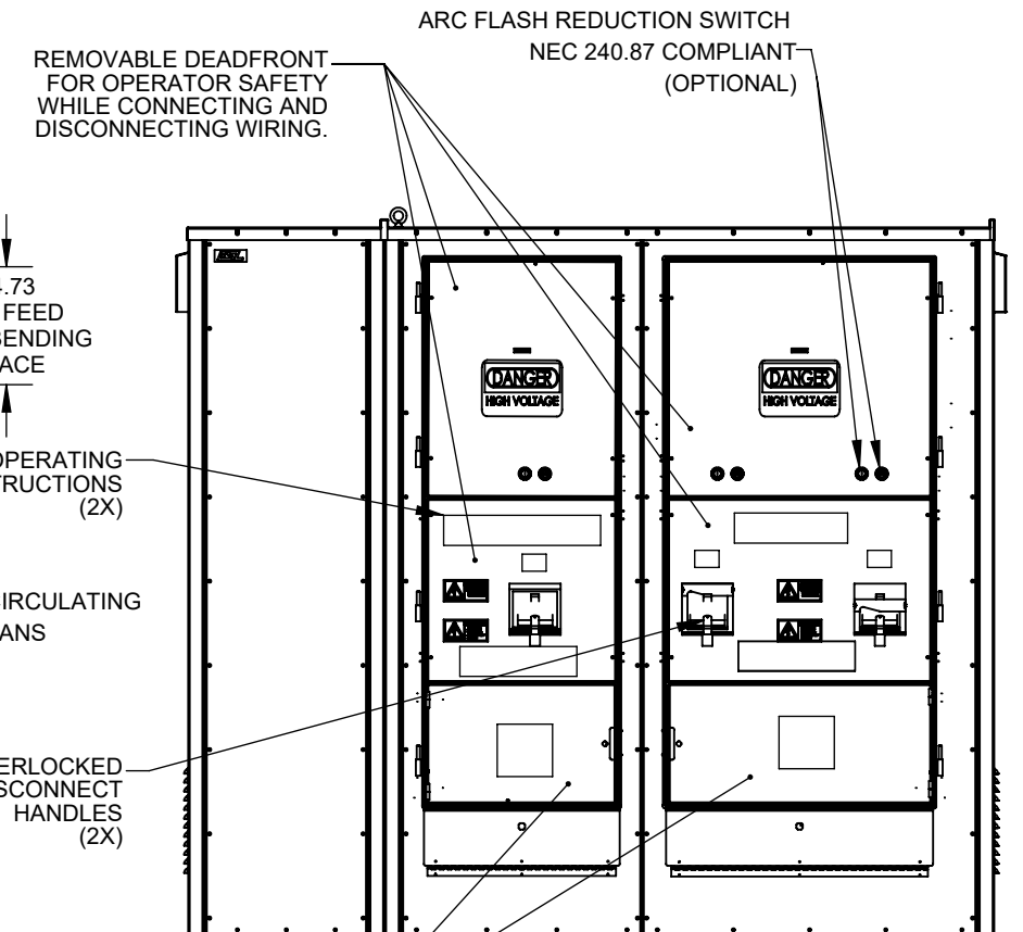
FRONT VIEW (DOORS REMOVED)
