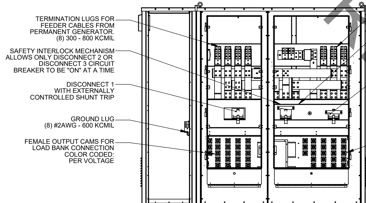
FRONT VIEW (DOORS AND DEADFRONTS REMOVED)
