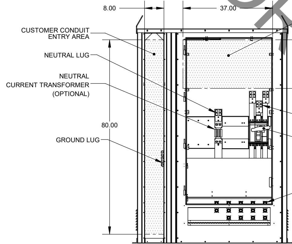
FRONT VIEW (DOOR AND DEADFRONT REMOVED)
